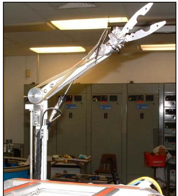
Figure 17 View of Gripper Extended
